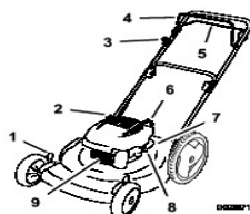
Figure 7 1. Cutting height lever 2. Oil fill/dipstick 3. Rear deck handle 4. Blade control lever 5. Self-propelled drive lever 6. Fuel tank cap 7. Air filter 8. Mower 9. Spark plug
